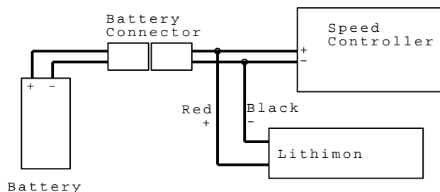
Fig. 1: Connecting Up
